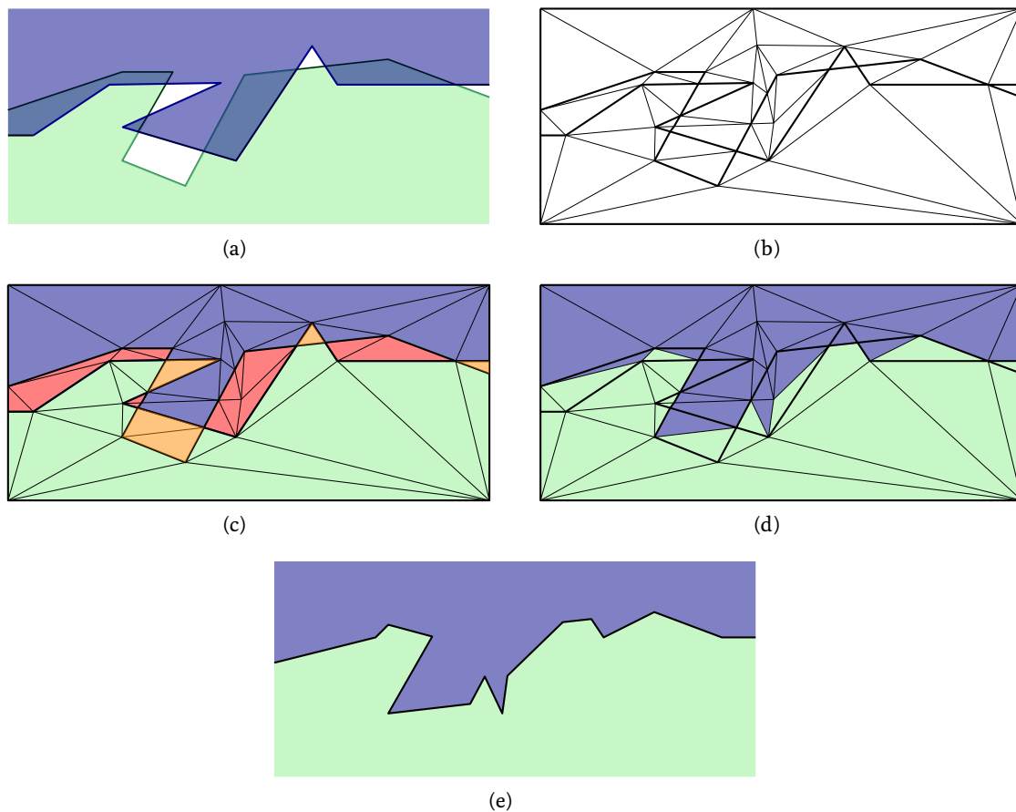
Figure 4: (a) Original dataset with two polygons (same as Figure 2). (b) The CT of the input polygons. (c) Labelling of the triangles: the colours represent the label of each polygon (orange = no label; red = 2+ labels). (d) Triangles are re-labelled such that each triangle has one and only one label. (e) The resulting alignment of the two polygons.
