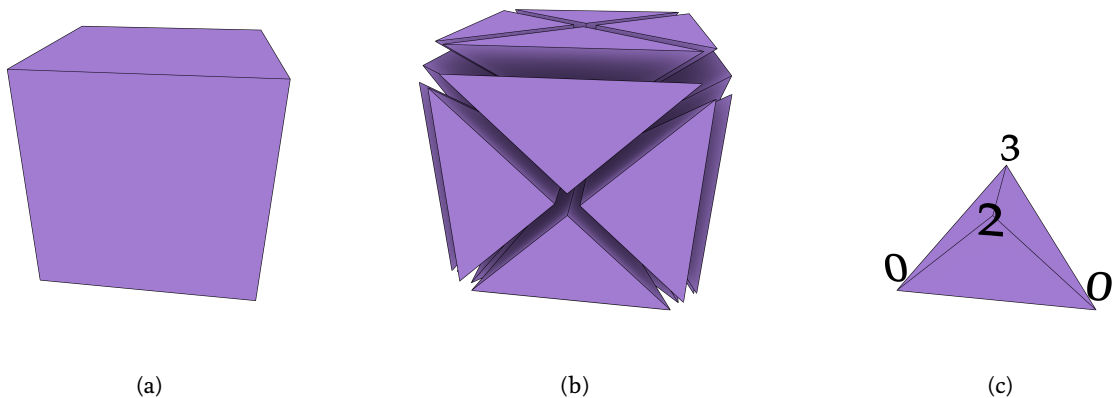
Figure 8: A 3D combinatorial map representation of a (a) cube consists of (b) 24 darts. (c) Each of these darts is defined by an incident edge-face-volume triplet. In this case, they are the lower front edge (between the os), front face (2) and the only volume of the cube (3). Note that there are also two possible orientations for such a map, which are not shown here.
