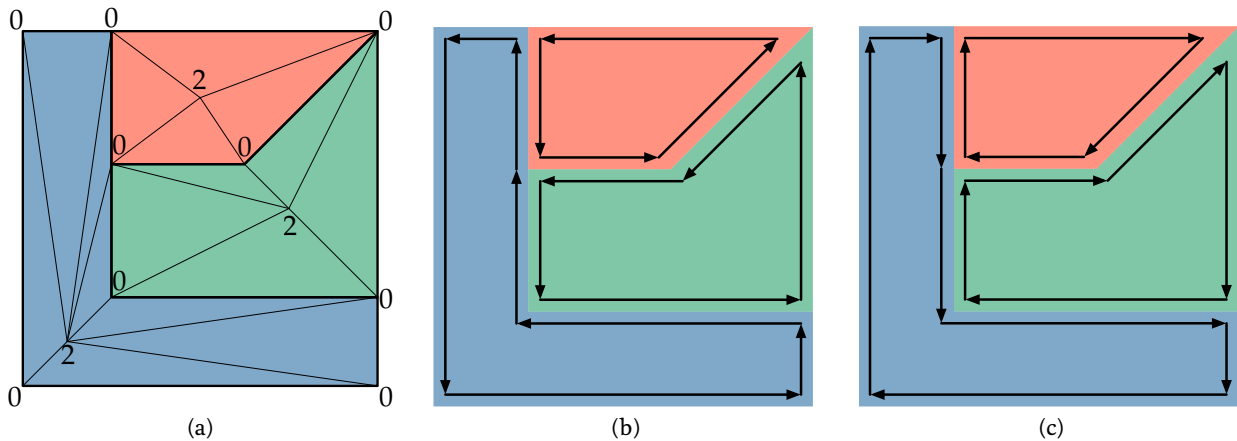
Figure 7: A 2D combinatorial map representing three polygons. (a) The underlying simplicial complex, where every triangle consists of two vertices (marked as o) at either end of an edge and a symbolic vertex for every face (marked as 2). (b) The combinatorial map that is generated by choosing a counterclockwise orientation for the polygons. (c) Same for the clockwise orientation. Darts are represented by triangles in (a) and arrows in (b) and (c).
