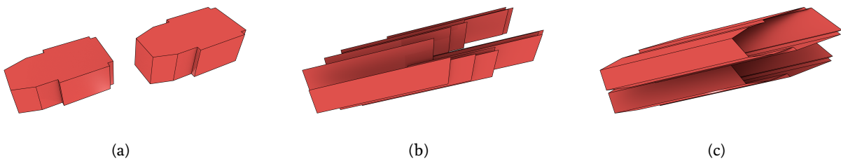
Figure 6: The polyhedron in Figure 3 can be extruded to 4D using the algorithm in Arroyo Ohori et al. [2015c]. The result is a single polychoron, whose faces are shown here in parts for clarity: (a) the faces in the two end volumes, (b) the lateral faces connecting corresponding vertical edges, and (c) the top and bottom faces connecting corresponding horizontal edges. Not shown here are the 16 polyhedra that are formed from these faces.
