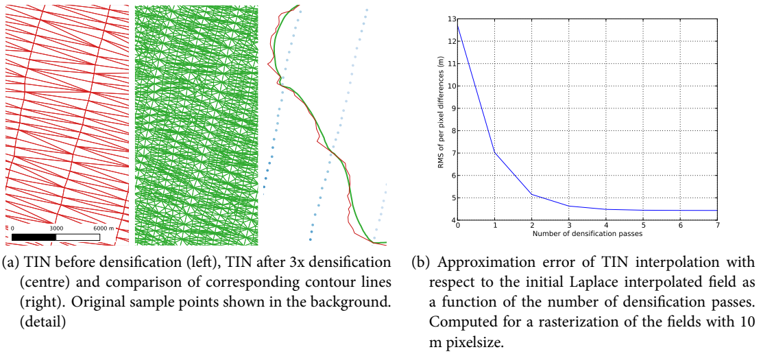
Figure 13: Densification illustrated on the Antilles dataset.
