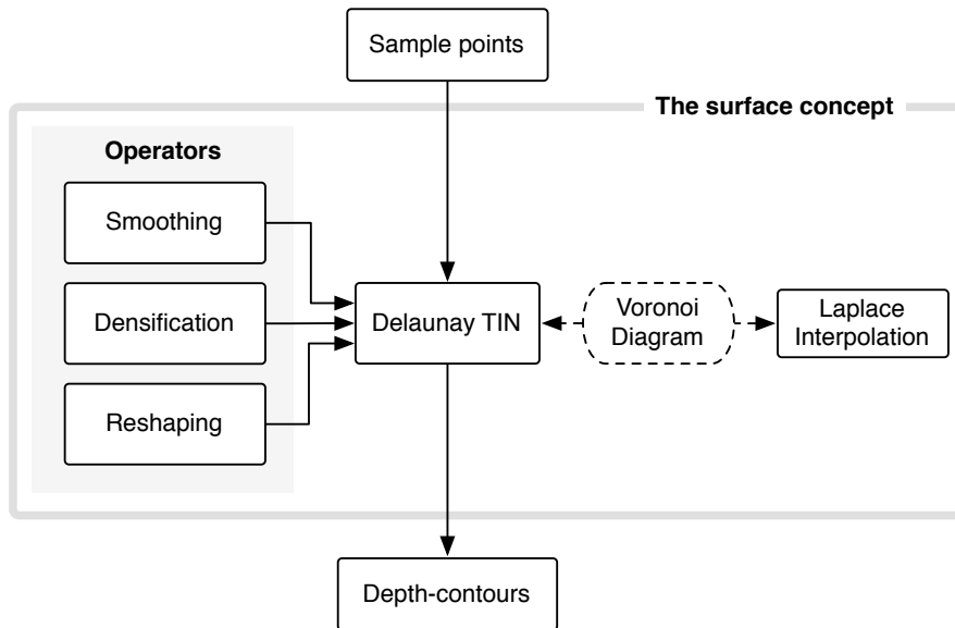
Figure 7: Overview Voronoi- and surface-based approach
