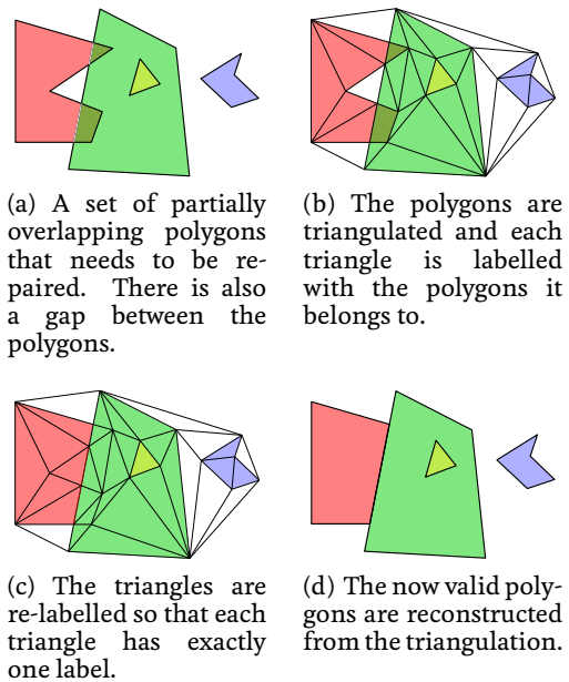
Figure 4: The steps to repair a planar partition.
