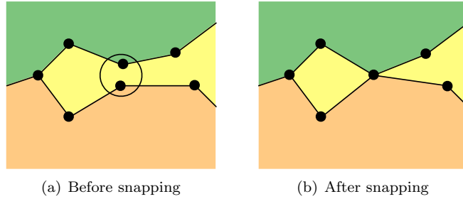
Figure 4: Polygons can be split by snapping, since some parts might be narrower than the threshold (encircled). While this result does not create an invalid result, it can change the number of polygons present and their topological relations, and can therefore be undesirable.
