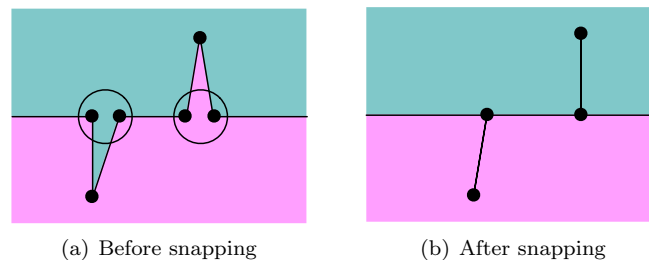
Figure 3: Spikes and punctures can be created by snapping, since the bases of these elongated forms (encircled) might be narrower than the threshold, but their lengths not.
