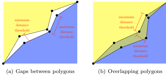
Figure 2: Defining a threshold for vertex and edge snapping. The threshold to use should be larger than the largest minimum distance between the matching boundaries, and smaller than the minimum distance between vertices of a single polygon.
